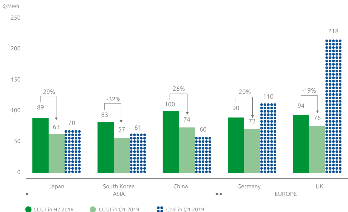
Average Levelized Cost of Energy of gas vs. coal (2018-2019)
